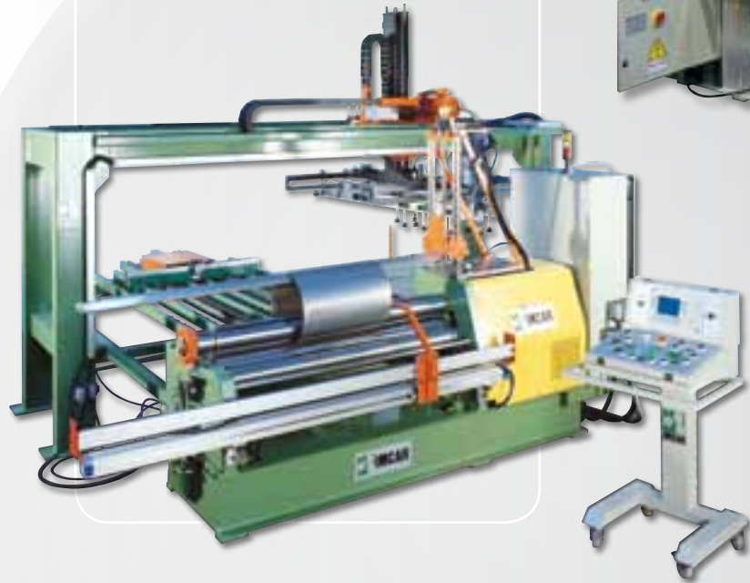
PALLET LINE
